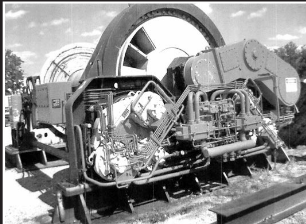
New motors installed on Rapp MHW-140 Winch approx. 2 years ago.
