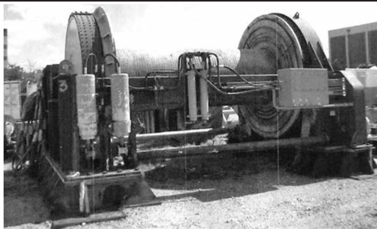
View of Rapp MHW-140 Multi Purpose Winch
